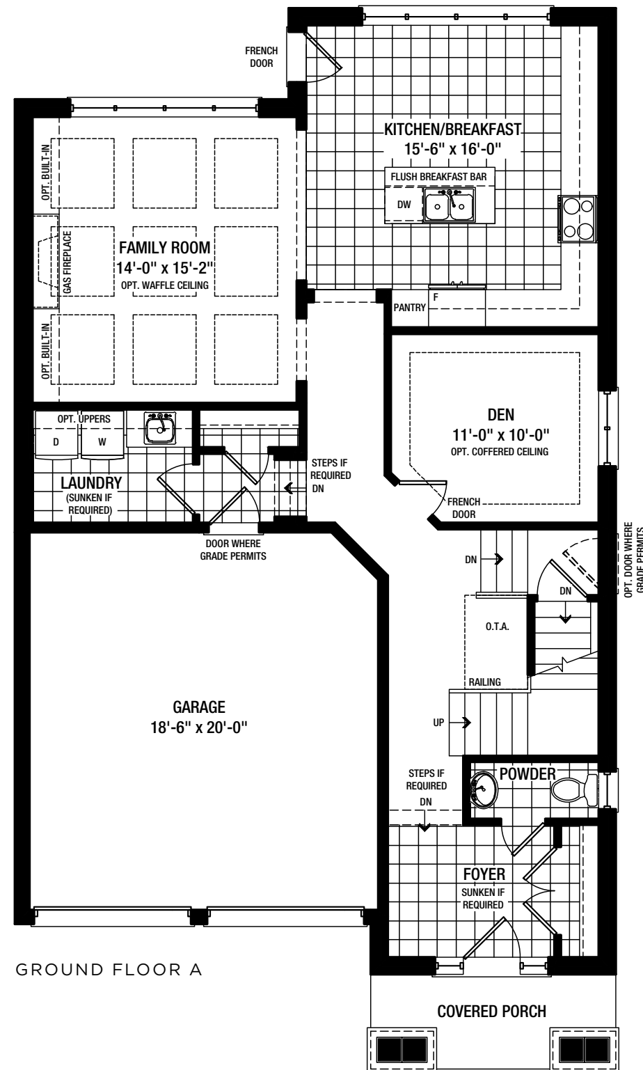
OPT. WALK-UP GROUND FLOOR A & B
