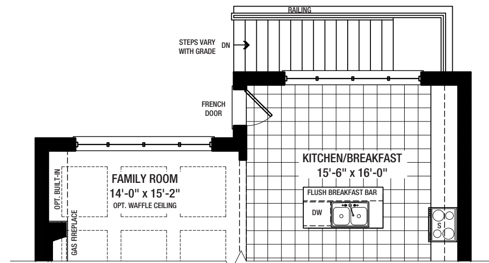
OPT. WALK-UP GROUND FLOOR A & B
