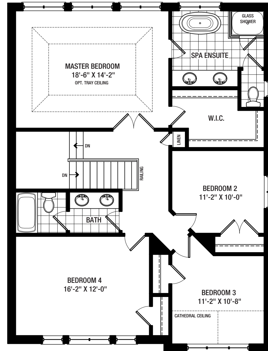
SECOND FLOOR A
