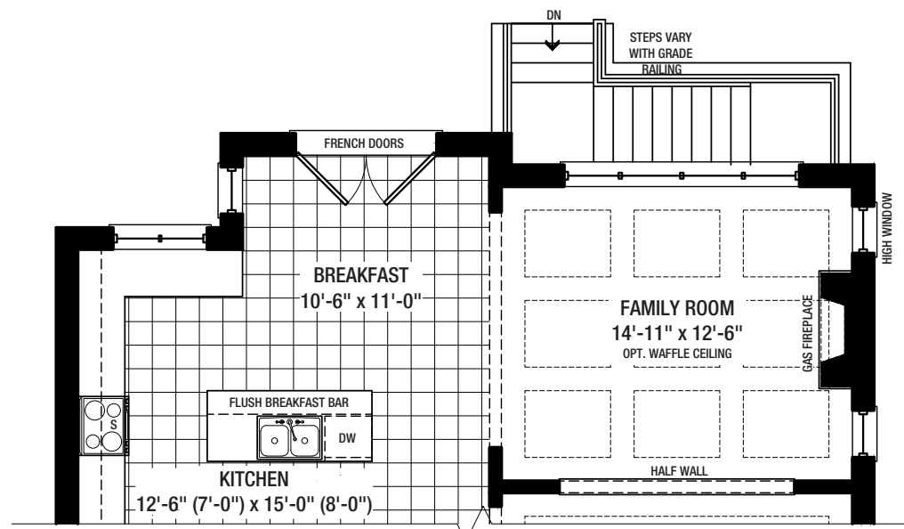
OPT. WALK-UP GROUND FLOOR A & B
