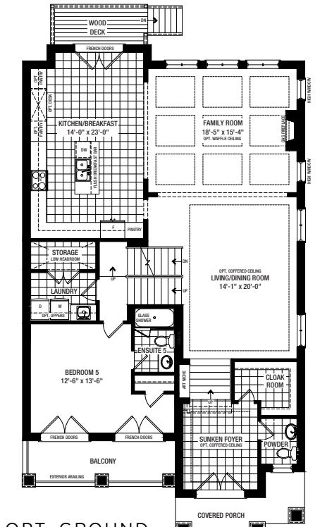
OPT. GROUND FLOOR A 5 BEDROOM PLAN
