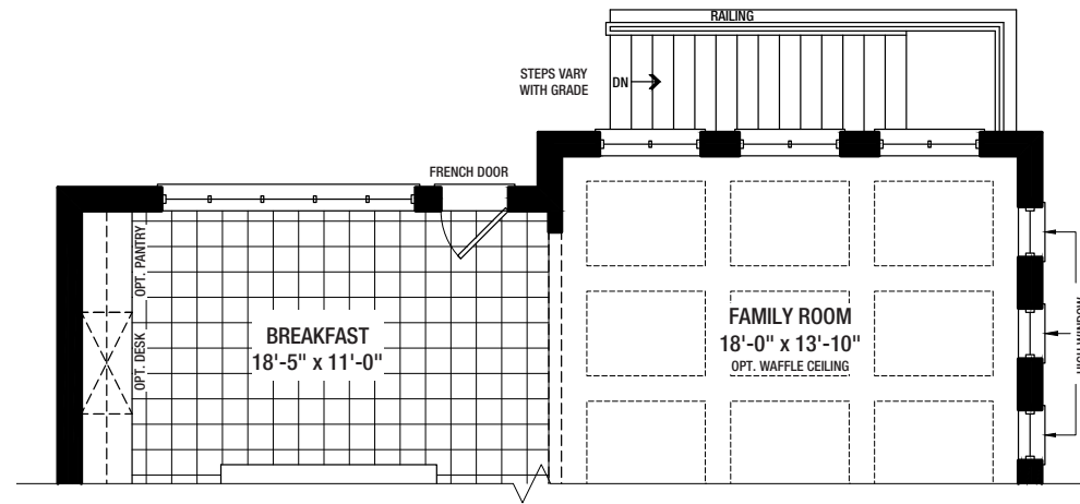
OPT. WALK-UP GROUND FLOOR A & B
