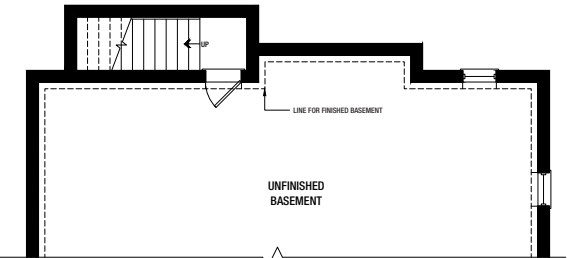
OPT. WALK UP BASEMENT A & B
